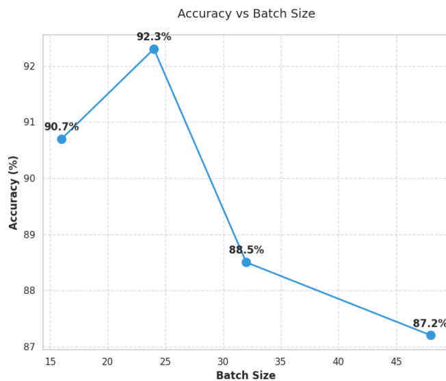
EfficientNet Hyperparameter Analysis
